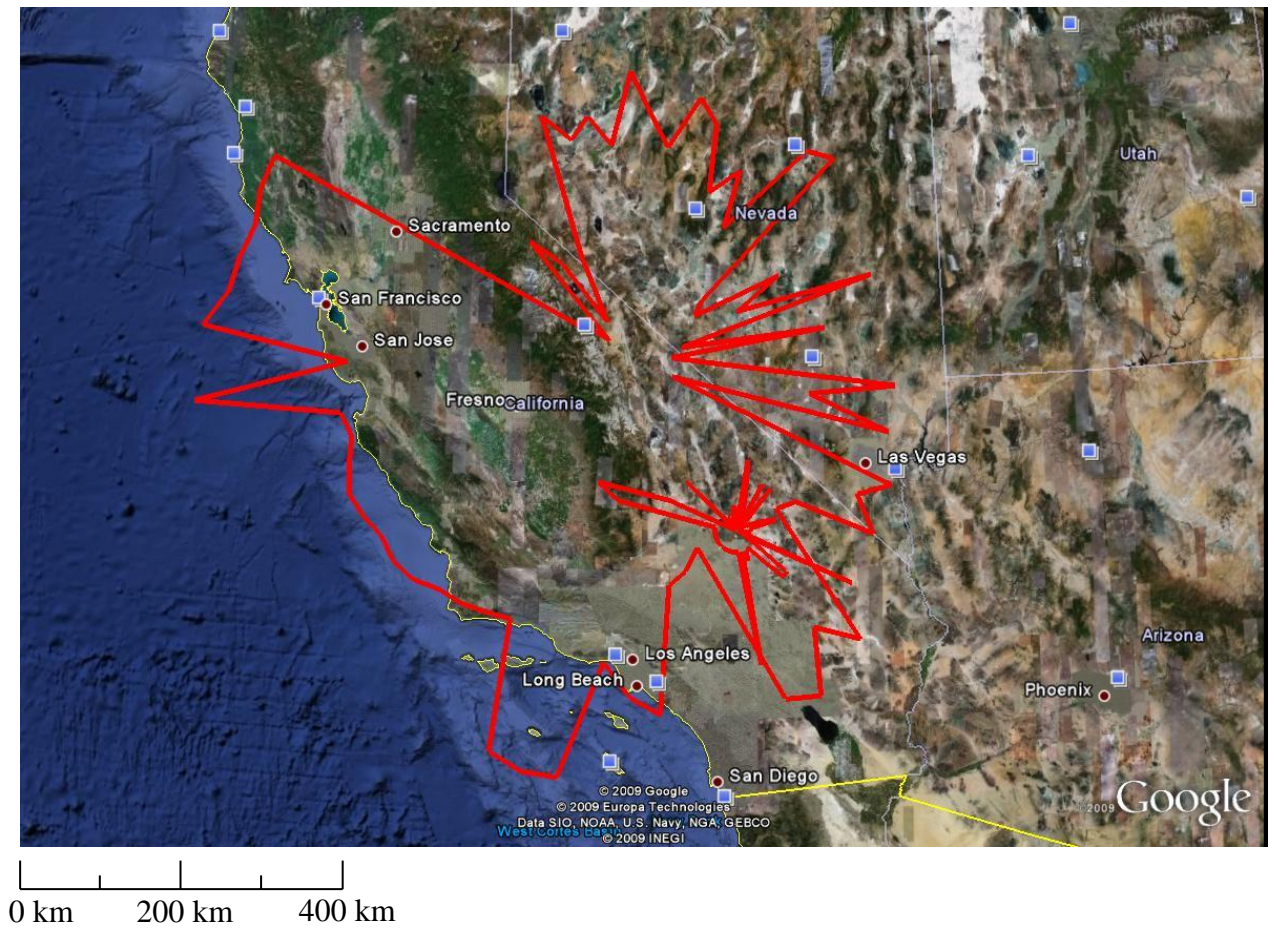
Figure 5. Owens Valley, CA and NASA Deep Space Network, CA 1660.5-1668.4 MHz Radio Astronomy Spectrum Contours
