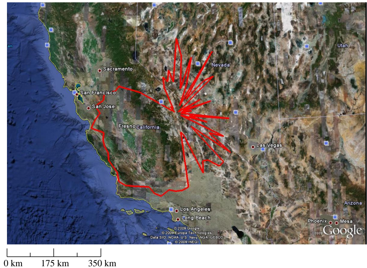
Figure 6. Owens Valley, CA 4990-5000 MHz Radio Astronomy Spectrum Contour
