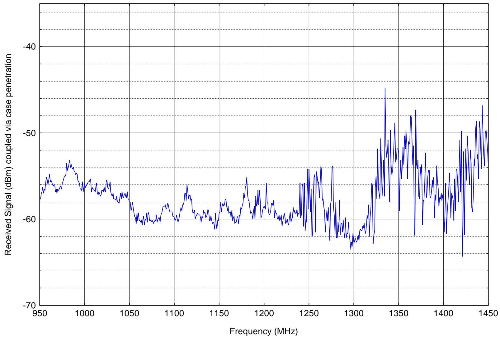
Figure 3. Earth station antenna w. 50-ohm load replacing feed; radar coupling
