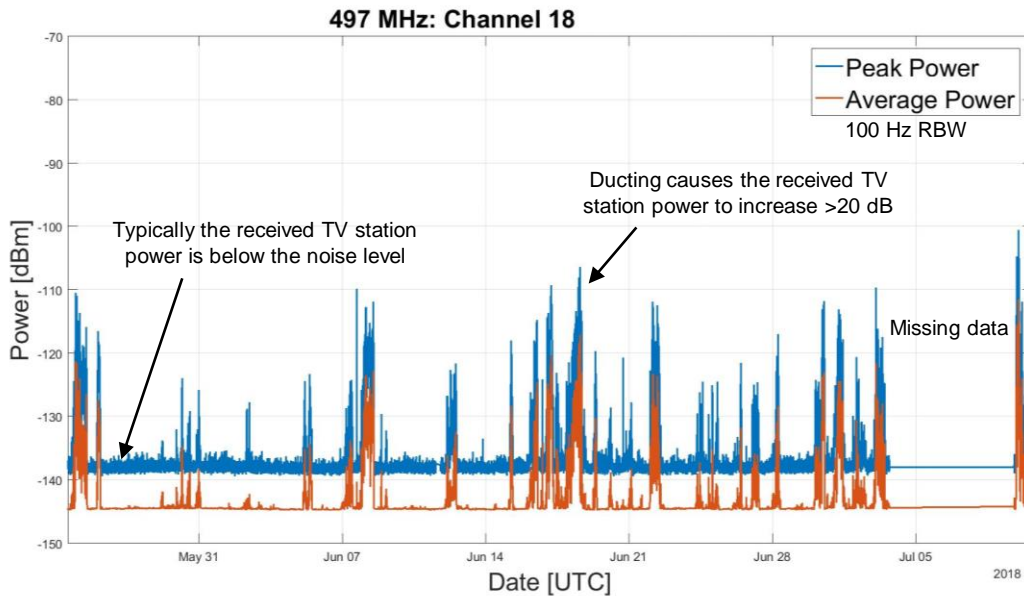
FIGURE 1. MEASURED TV SIGNAL POWER OVER A SEVERAL MONTH PERIOD AT OCEAN CITY, NJ SHOWING SIGNIFICANT POWER VARIATION DUE TO ANOMALOUS PROPAGATION (DUCTING)
