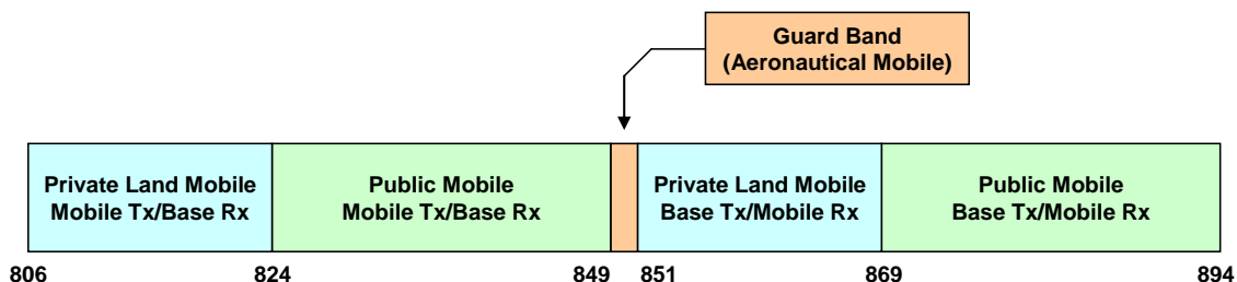
Figure 8 – The 800 MHz land mobile band and associated guardband
